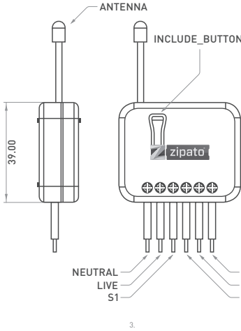
FIGURE 1 Dimensions [unit: mm]
